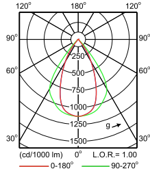
IFPS_4MX850 G3 581 1xLED66S/840 PSD NB- Polar Normal (separate)
