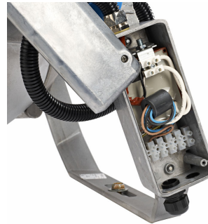
Electrical connection box equipped with e-ignitor
