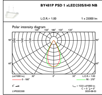
OFPC1_BY481PPSD1xLED250S840NB
