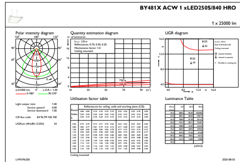
IFGU1_BY481XACW1xLED250S840HRO
