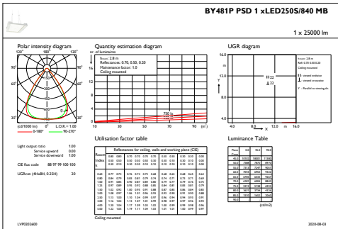
IFGU1_BY481PPSD1xLED250S840MB
