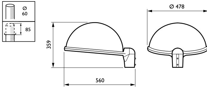
BRP775 LED49-4S/740 PSD DW50 PGR BK D9
