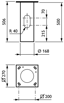
ZCB500 TUBE L500
