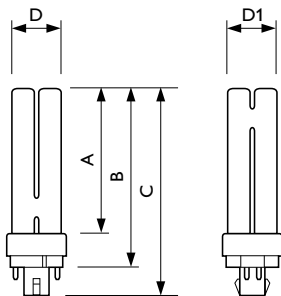
PL-C 18W/840/4P
