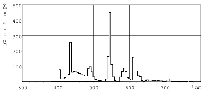
LDPB_PLC4P_865-Spectral power distribution B/W
