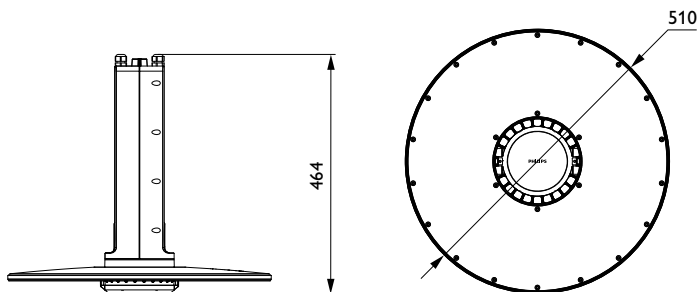
BY122P G4 LED250S/840 SRD WB H4
