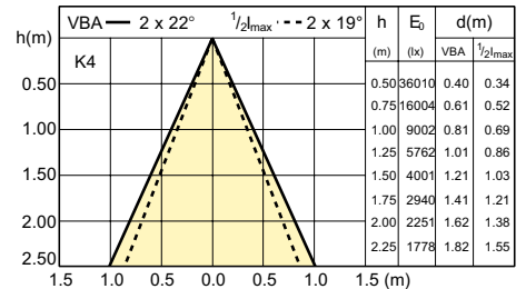
LDBE_CDM-R111_70W_40D-Beam diagram
