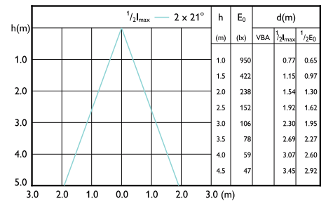
GU10 7.5-80W 650lm 2700K GU10 D 15khrs
