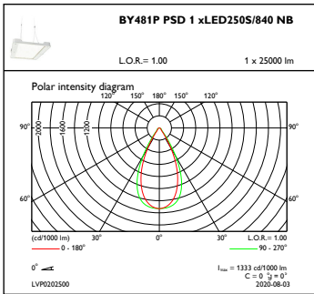
OFPC1_BY481PPSD1xLED250S840NB
