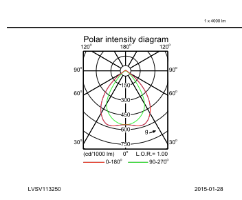
IFPC_4MX900 G3 491 1xLED40S/840 PSU WB-Polar Indoor (combined)
